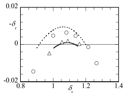
Figure 2. Variations of the amplification rate \delta_i of disturbances in a Poiseuille flow at Re=4000 (triangles) and Re=5000 (circles) as a function of the disturbance wave number \delta_r . One of the walls is smooth and the other has wavy form with the roughness wave number \alpha=1.02 and the amplitude S=0.04 .
