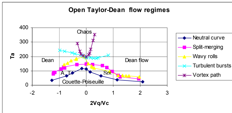
Fig. 3 Open Taylor-Dean flow regimes (A.T.: axially translation motion; Spi.: Spirals)
