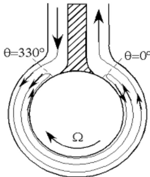
Fig.1 Sketch of the flow system
