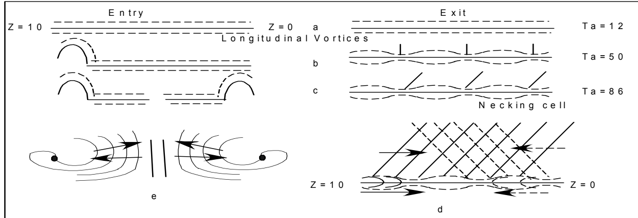
Fig.2 Rise and growth of the entry and exit instabilities for \tau=0
