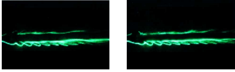
Figure 2. Results of the experiment - flow visualisation for A=5 and f/f_{nat} = 4 (left) and for f/f_{nat} = 5 (right)
