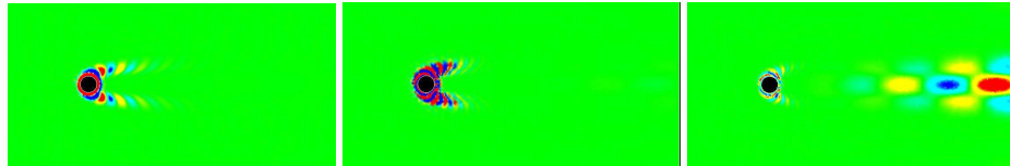
Figure 3. POD mode 1,3 and 5 vorticity (-5,5) for “fully controlled” case
