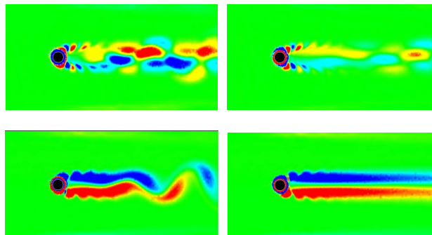
Figure 1. Disturbance vorticity (-5,5) for the fully controlled case ( Re = 100 , A = 5 , f/f_{nat} = 4.5 ), for time T = 33.6 (left) and T = 200 (right) and respective sum of the disturbance with the steady flow solution.
