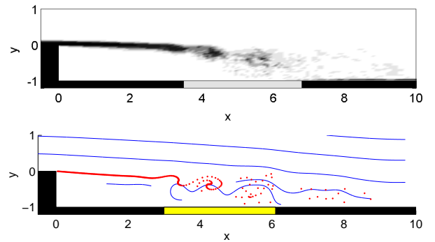
Fig. 3: Numerical simulation (top) and low-dimensional vortex model with \approx 300 vortices (bottom) of the flow around a backward-facing step at Re_h = 4000 . The top figure illustrates the vorticity distribution of a snapshot. The figure at the bottom indicates vortex locations by red dots. Regions of upstream velocity close to the wall are marked by grey bars.
