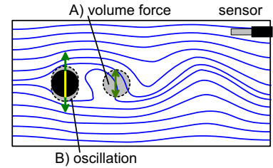
Fig. 1: Streamlines of the von Kármán vortex street in the wake of a circular cylinder at Re = 100 . Two different actuators are investigated: A) a local volume force, and B) oscillations of the cylinder. The state of the flow is monitored by a single hotwire probe.
