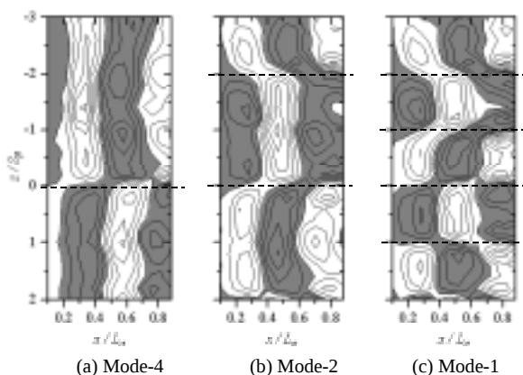
Fig.4 Contour maps of streamwise velocity fluctuations in xz -plane at y = 0 and supplied voltage = 70 V (IFS)
