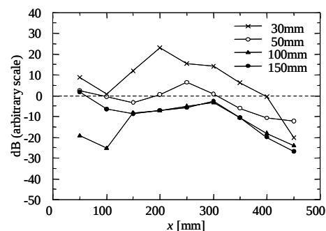
Fig. 6 Variation of peak level with plates of different vertical lengths and x locations (RTRI)
