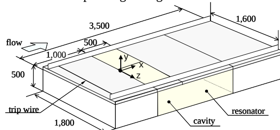
Fig.2 The model with a cavity (RTRI)
