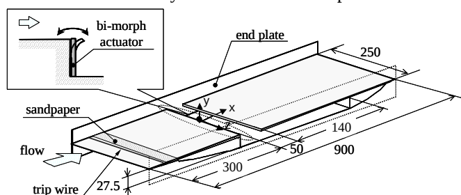
Fig.1 The model with a cavity (IFS)
