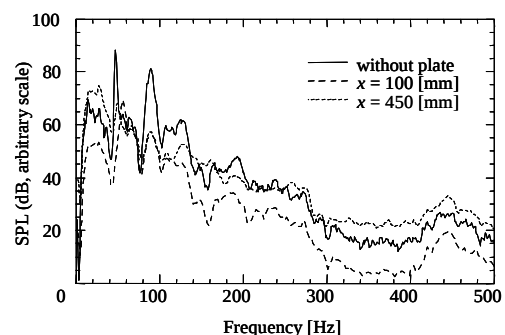
Fig.7 Sound suppressing effect with the plate (vertical length = 100 [mm]) at x = 100 and 450 mm (RTRI)
