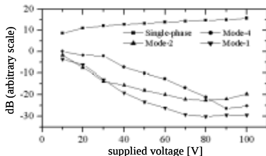
Fig. 3 Noise suppression effect of bimorph actuators (IFS)
