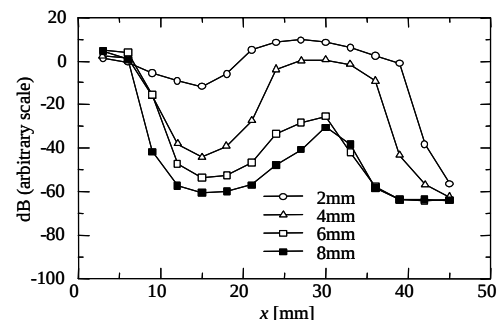
Fig.5 Variation of peak level with plates of different vertical lengths and x locations (IFS)
