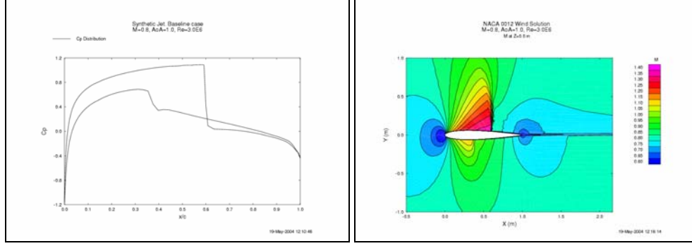
Figure 1: Computed Pressure Distribution and Mach Contours for Flow Past a NACA 0012 Airfoil at M=0.8 , Re = 3.0 \times 10^6 , \alpha=1.0^\circ without Synthetic Jet.
