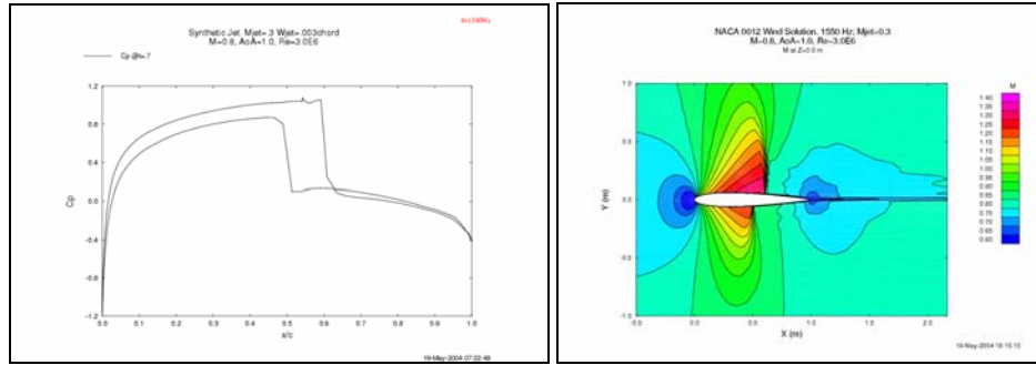
Figure 2: Computed Pressure Distribution and Mach Contours for Flow Past a NACA 0012 Airfoil at M=0.8 , Re = 3.0 \times 10^6 , \alpha=1.0^\circ with Synthetic Jet, Jet Width = 0.003c , M_j = 0.3 , f = 1550 Hz.
