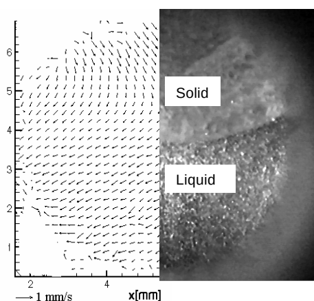
Figure 3: Convective processes during melting of Ice I
