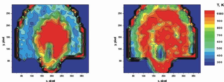
Fig. 1. Instantaneous temperature maps reconstructed by CAT with Radon integral equation using two-projectional DSP
