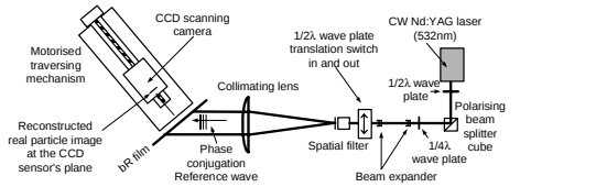
Figure 3: Reconstruction of two sequentially multiplexed polarization holograms using circular polarization wave.
