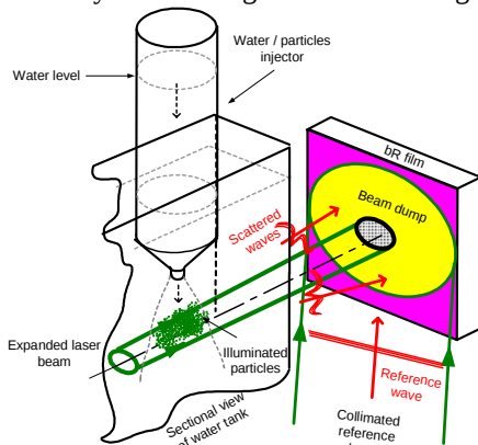
Figure 1: Schematic of recording a hologram on bR using forward scattering on off axis geometry.
