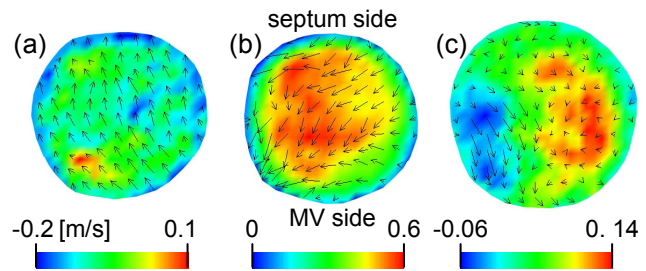
Fig. 3 Vector and counter plots of the flow at the plane 1.3 cm above from the aortic valve constructed from MR data. (a) early, (b) mid, (c), end systole.
