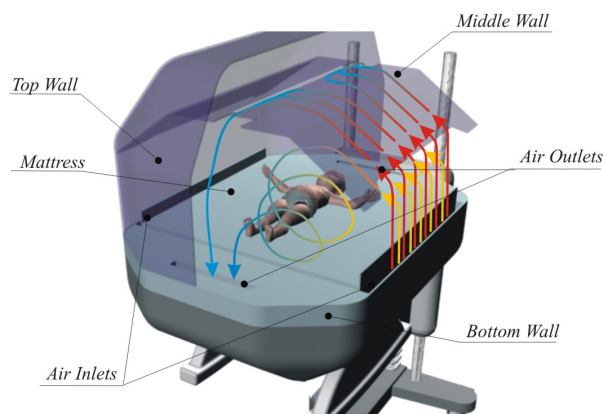
Figure 1. Modelled newborn infant placed within an infant incubator.
