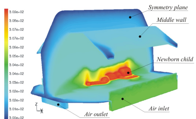
Figure 2. Perspective view of the temperature field.
