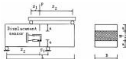
Fig.2 Four-point-shear specimens
