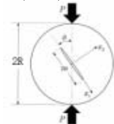
Fig.1 Brazilian disk specimens
