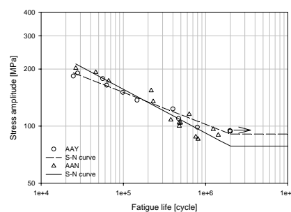
Fig. 2 S-N curves for annealed (AAY) and as-welded (AAN) specimens
