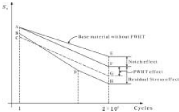
Fig. 3 Schematic diagram of S-N curves
