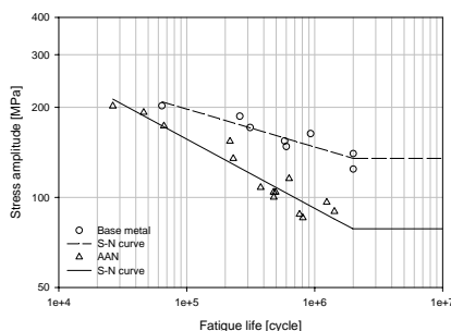
Fig. 1 S-N curves for base material and as-welded (AAN) specimens
