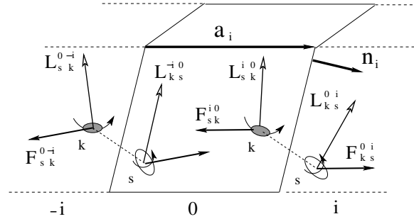
Figure 2. A cell of a crystal. Discrete model
