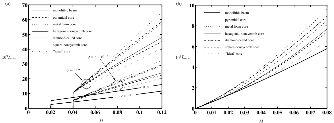
Figure 1. A comparison of the maximum blast impulse sustained by monolithic beams and by optimal designs of sandwich beams. (a) Water blast and (b) air blast.
