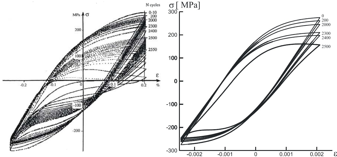
Low cycle fatigue stress strain pattern for AISI 316L: Dufailly's experiment (left) and numerical simulation (right)
