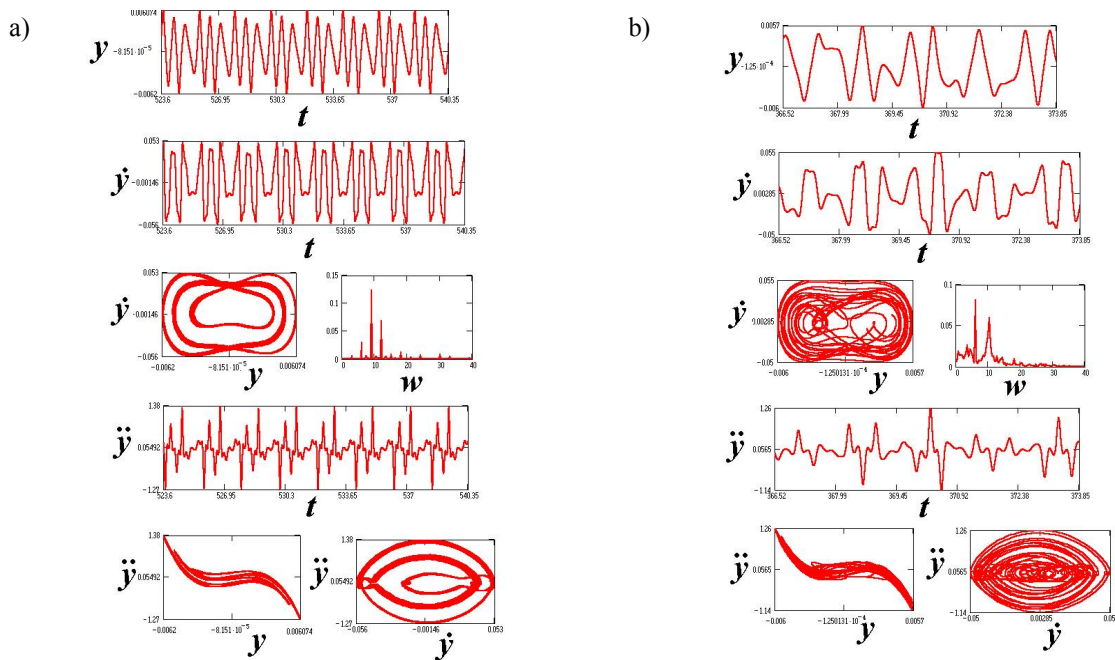
Figure 2. Time characteristics and phase trajectories of the system under consideration ( m = 3 ; \varepsilon = 0.5 \text{ s}^{-1} ; \alpha = 408 \text{ s}^{-2} ; \beta = 7660000 \text{ m}^{-2} \text{ s}^{-2} ; F_1 = 0.15 \text{ ms}^{-2} ; F_2 = 0.075 \text{ ms}^{-2} ): a) combinatorial oscillations; b) chaotic oscillations.
