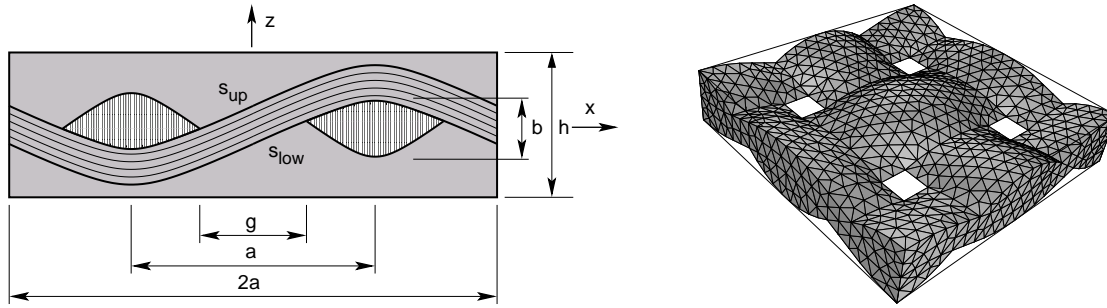
Figure 1. Idealized Periodic Unit Cell, (a) Geometrical model, (b) Example of finite element mesh
