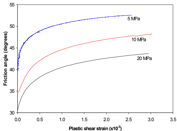
Figure 2. Friction of Berea sandstone.
