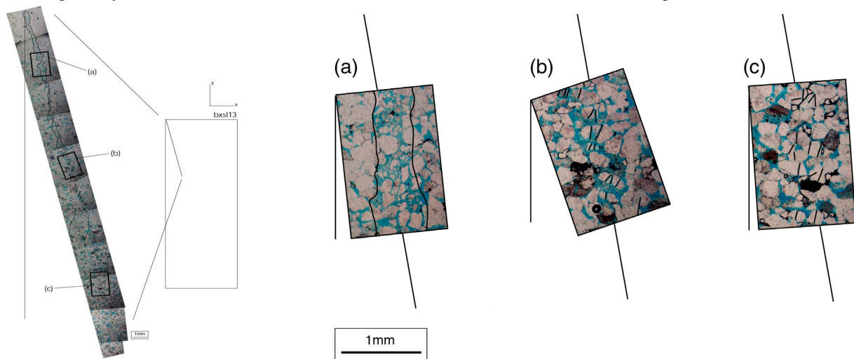
Figure 3. Shear band in Berea sandstone at 5 MPa confinement.
