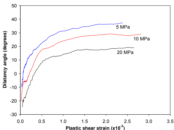
Figure 1. Dilatancy of Berea sandstone.
