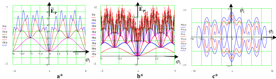
Figure 2. Multistep-coupled heavy rotors free nonlinear dynamics visualizations (Multipliers). a* and b* Potential energy curves families. c* Phase homoclinic trajectories portraits (constante energy curves). Homoclinic orbits layering for conservative system.
