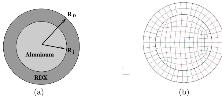
Figure 1: Schematic of (a) an explosively coated aluminum grain and (b) the computational grid within a grain used for the representative simulation.
