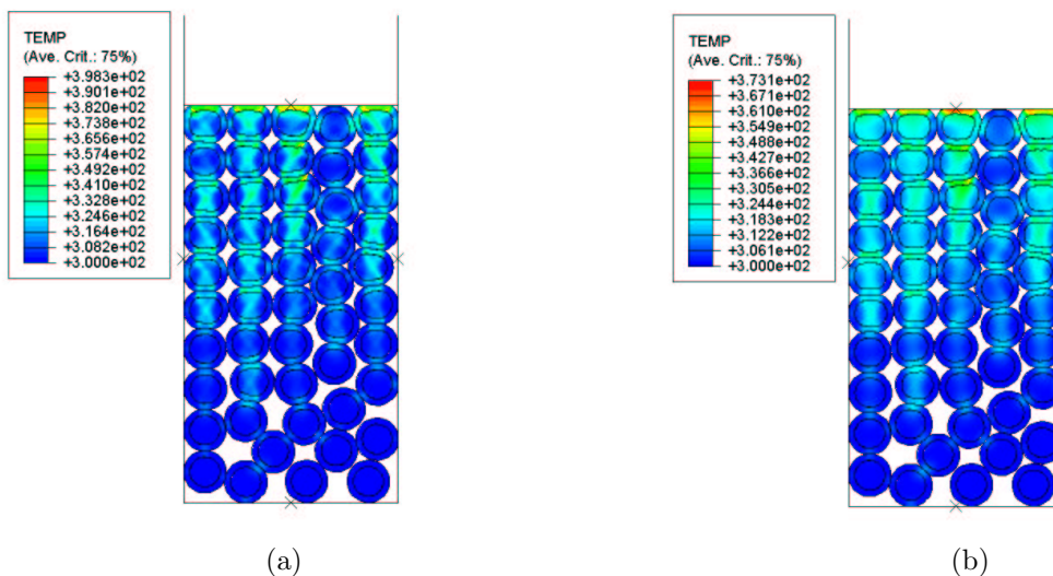
Figure 2: Predicted temperature field for explosively coated aluminum grains for a piston speed of 150 m/s: (a) without thermal conduction and (b) with thermal conduction.
