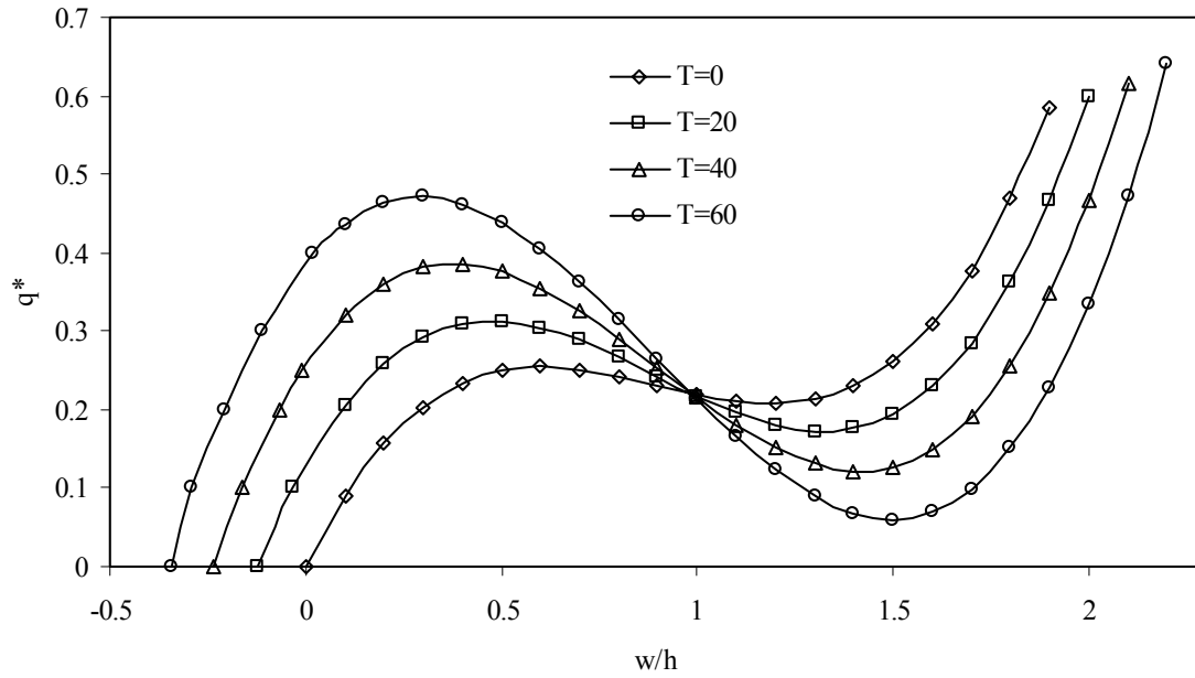
Figure 1: Response of doubly curved shell panel [0/90/0] subjected to thermo mechanical loads. ( a/b = 1 , R_1/R_2 = R , q^* = q_0 R_2/E_2 h^2 , E_1 = 25E_2 , G_{12} = G_{13} = 0.5E_2 , G_{23} = 0.2E_2 , \nu_{12} = 0.25 , \alpha_2/\alpha_1 = 3 )
