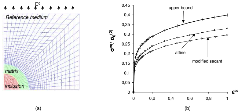
Figure 1. (a) Example of 2D mesh used. (b) Effective behaviour of a two-phase, power-law type, particulate composite with 30% inclusions and a contrast of 5.
