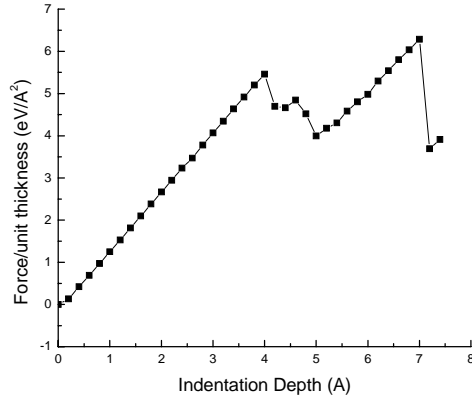
Figure 1: The force per unit thickness versus indentation depth for the simulation
