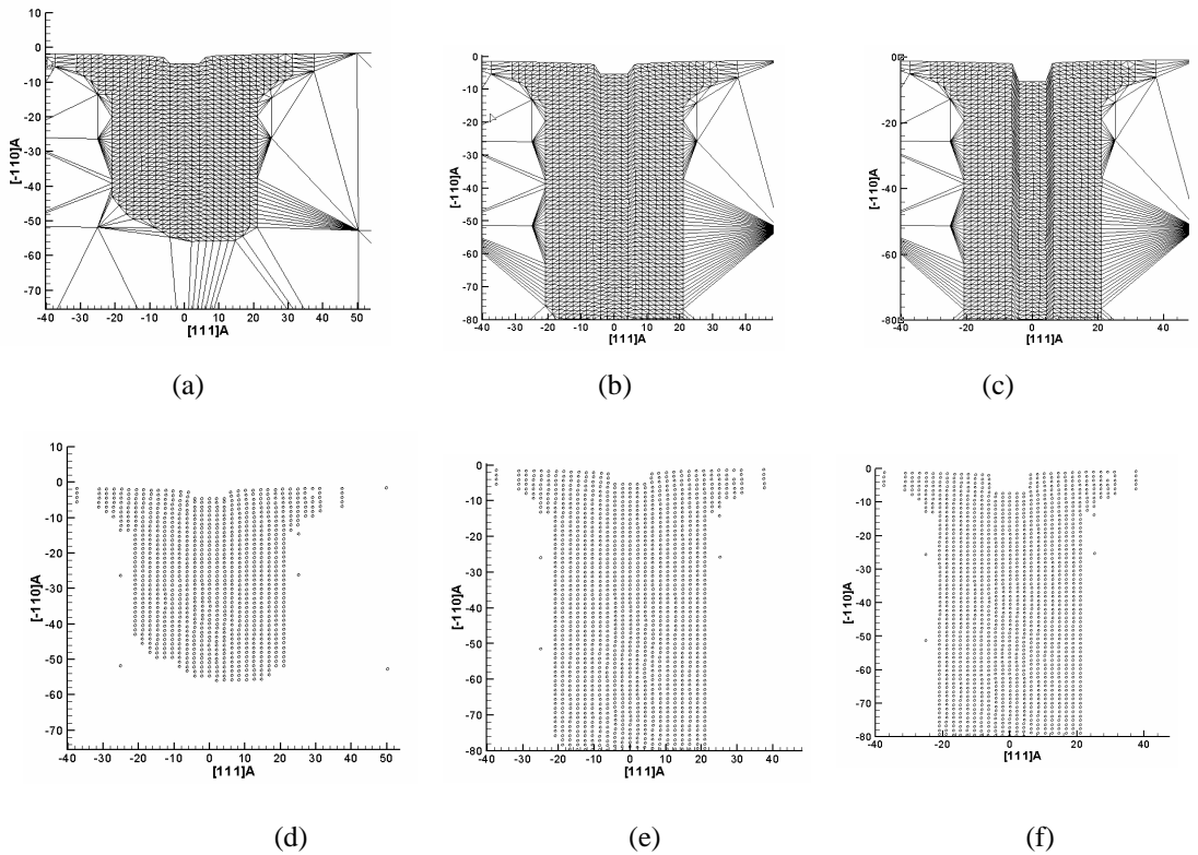
Figure 2: Three snapshots of the mesh under indenter (a) immediately before the first emission, (b) after emission of dissociated dislocations from both ends of the indenter and (c) final dislocations. Frames (d), (e) and (f) show the corresponding scatter plots.
