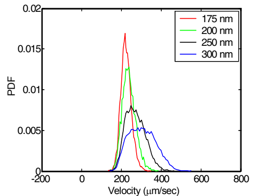
Figure 4. Simulated velocity distributions of 300-nm particles at a shear rate of 1400 \text{ sec}^{-1} with four different observation depths.
