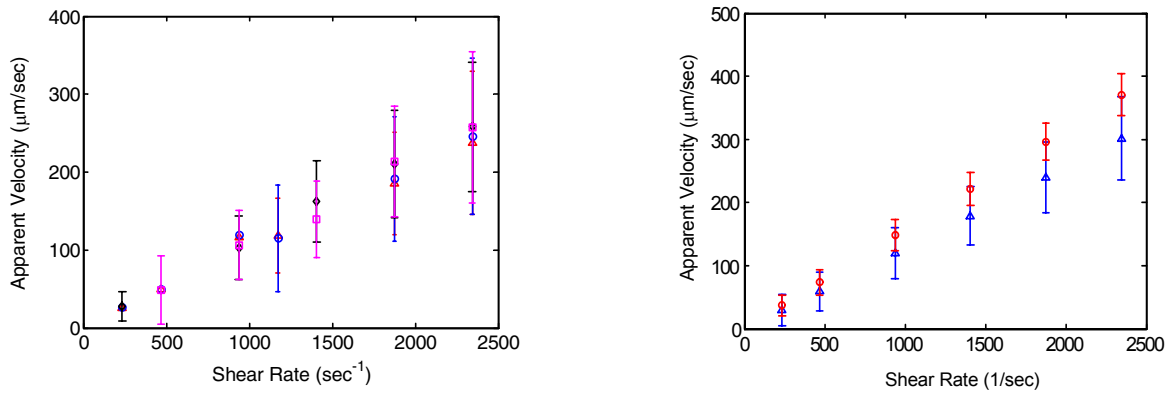
Figure 3. Apparent velocity vs. shear rate. The left frame shows the experimental results (hydrophilic: 200-nm particles – red; 300-nm particles – black / hydrophobic: 200-nm particles – blue; 300-nm particles – pink) while the right frame shows the Monte Carlo simulation (200-nm particles – blue; 300-nm particles – red) at observation depth = 175 nm.
