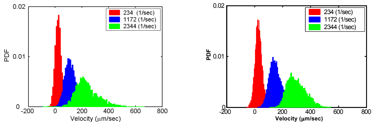
Figure 2. Distributions of velocity at three shear rates. The left frame shows the experimental results while the right frame shows the corresponding result from the Monte Carlo simulation (using an assumed observation depth of 175 nm).
