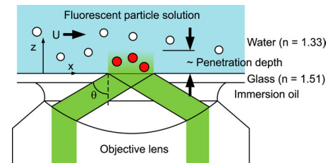
Figure 1. Schematic of objective-based TIRFM setup.
