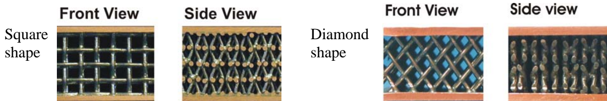
Figure 1. Two prototype textile laminate heat exchangers.
