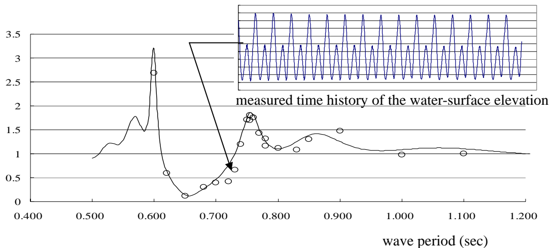
Figure 2 The frequency response characteristics of the water-surface elevations between the two rows of the array of 2x8 cylinders in head waves (solid line: linear-theory calculation, circles: experimental results)
