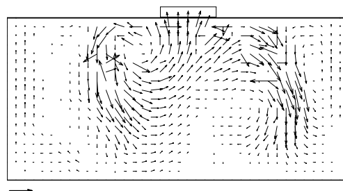
Figure 3. Velocity vectors map, Re = 10 .
