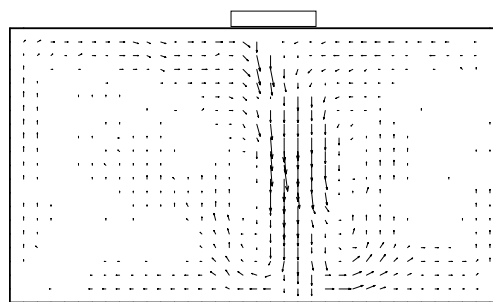
Figure 2. Velocity vectors map, Re = 0 .
