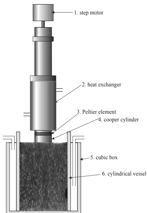
Figure 1. Schematic view of experimental equipment.
