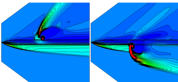
(a) Case 3 (b) Case 4 Fig. 2 C_p contour at the symmetry plane
