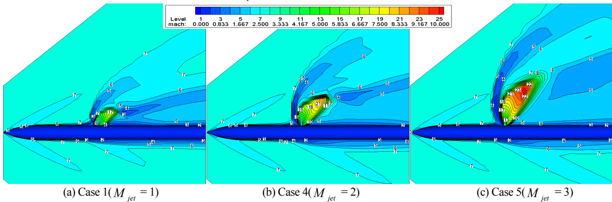
Fig. 8 Mach number Contour at the symmetric plane
