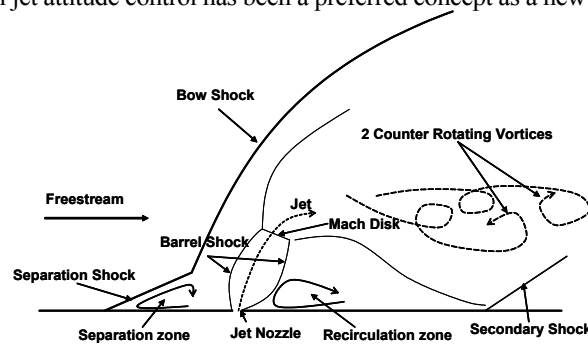
Fig. 1 Complicated flow structure around jet nozzle
