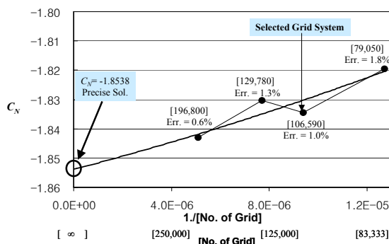
Fig. 4 The result of grid density test
