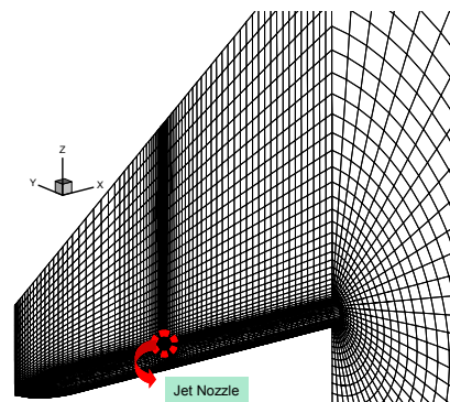
Fig. 5 Selected grid system ( 95 \times 34 \times 33 )
