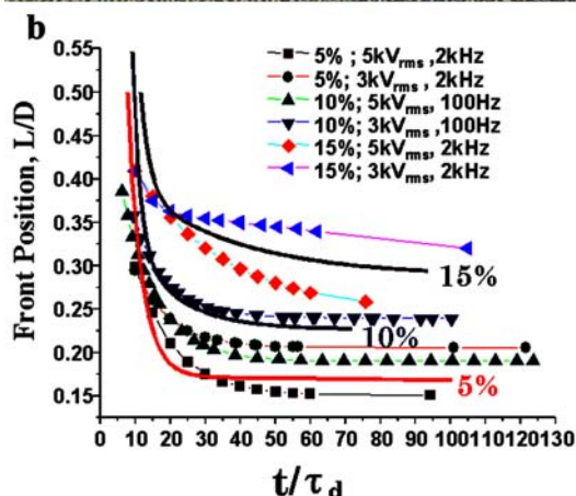
Figure 2. (a) The photo illustrates how the front location was measured; HV and GR refer to the high-voltage and grounded electrode respectively. (b) The experimental data (symbols) and computational results (solid lines) for the front propagation in 5, 10, and 15% (v/v) suspensions [8].
