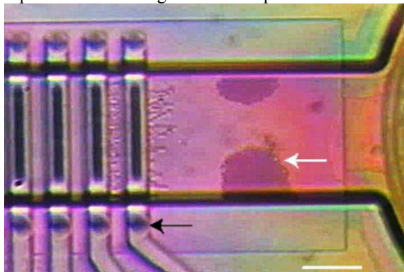
Figure 1. Dielectrophoretic (10Vptp, 15MHz) separation of bacterial cells and beads. The cells adhere to the energized electrode (black arrow) while the beads experience negative dielectrophoresis accompanied by a phase separation (white arrow). The flow is from right to left. Scale bar = 20 \mu\text{m} [6].
