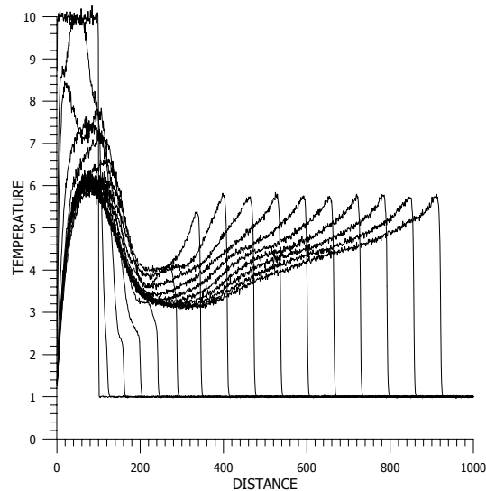
Fig. 1. Formation of a plane detonation wave without influence of walls.
