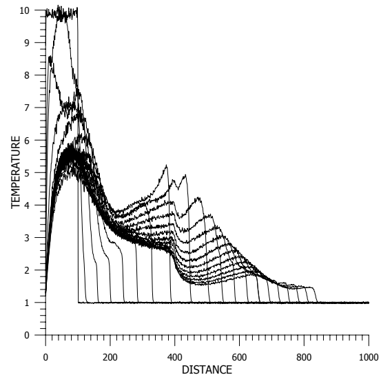
Fig. 2. Formation and decay of a detonation wave in a pipe.
