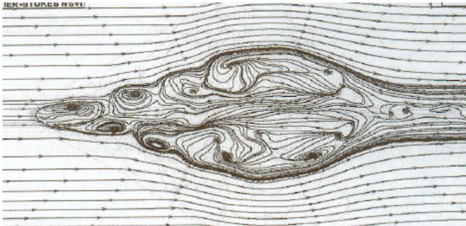
Fig. 1: Streamlines for normal shock-vortex interaction for Ma_{\infty} = 1.6 and Re_{\infty} = 1.5 \cdot 10^3 ; obtained with solution of Navier-Stokes equations.
