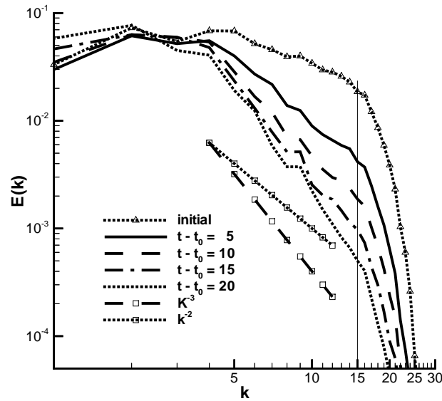
Figure 2. TNS: Energy spectrum at different time for Re = 4 \times 10^{15} , \Omega = 20 . Dotted line with deltas: initial condition; solid line: t - t_0 = 5 ; dashed line: t - t_0 = 10 ; dashed-dotted line: t - t_0 = 15 ; dotted line: t - t_0 = 20 ; dashed line with squares: k^{-3} spectrum; dotted line with squares: k^{-2} spectrum.
