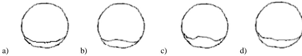
Figure 1: Sequence of instantaneous interface shapes. Pipe inclination 10^\circ , U_{LS} = 0.1 \text{ m/sec} , U_{GS} = 0.1 \text{ m/sec} .
