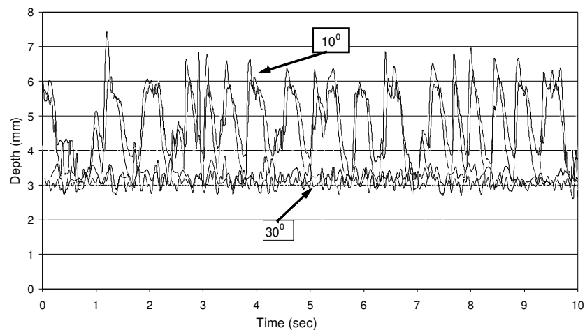
Figure 2: Instantaneous liquid film depth at the vertical diameter in the pipe cross-section derived from the recorded boroscope images (thin line) and measured by a capacitance probe (thick line). Flow rates as in Fig. 1.
