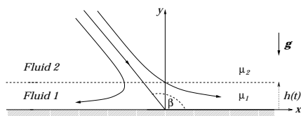
Figure 1: Planar two-fluid stagnation-point flow.
