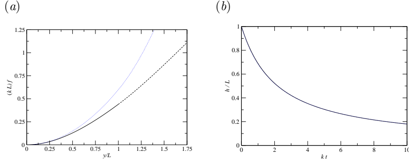
Figure 2: \lambda = 0.5 , h(0) = L = 1.0 : (a) The stream function f_j(y) at kt = 0 . The solid line corresponds to fluid 1, and the broken line corresponds to fluid 2. The dotted line is the Stokes solution. (b) h(t) versus kt for the quasi-steady (solid line) unsteady (dotted line) solutions.
