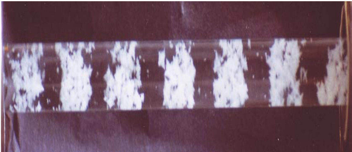
FIG.1 Banding phenomenon of \text{NH}_4\text{Cl} crystals in a supersaturated solution
