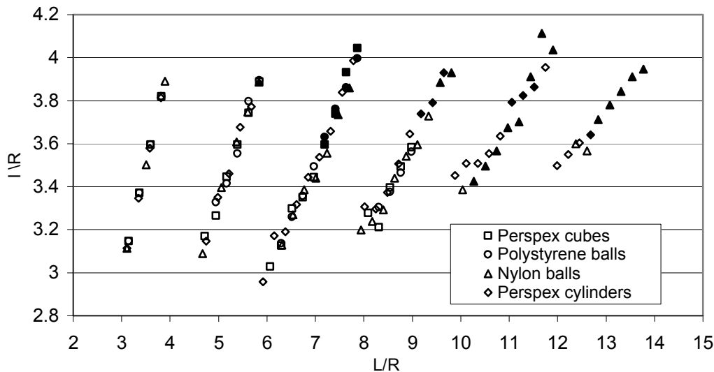
FIG. 2 A compendium of all data gathered in the investigation of the dependence of periodic length ( l ) on tube length ( L ) for particles suspended in water (full markers represent observed oscillations between two possible band patterns). The coordinates are scaled by tube radius in-order to manifest general features of the banding phenomenon.
