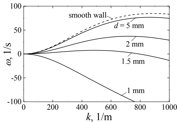
Figure 1. Disturbance growth rate for a film on vertical wall with rectangular grooves. Water, h^*=200 \mu\text{m} , shear stress 1 \text{ N/m}^2 .
