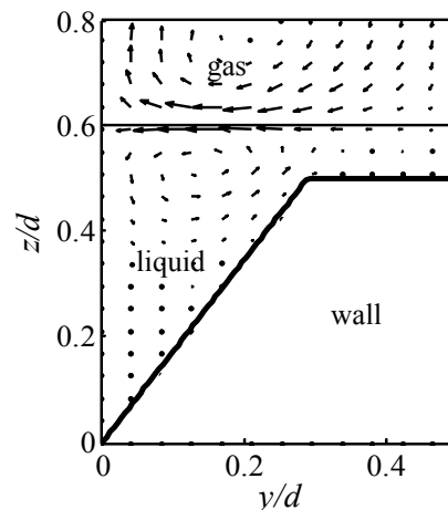
Figure 2. Thermocapillarity-induced velocity field in a film on a grooved wall.
