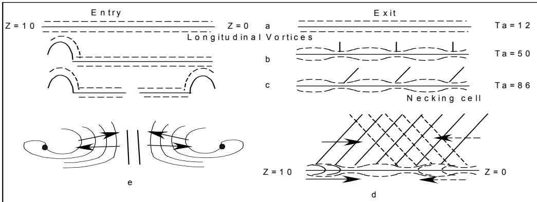
Fig.2 Rise and growth of the entry and exit instabilities for \tau=0
