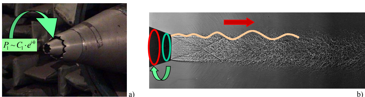
Fig.1 Non-adaptive and adaptive noise control: a) transformation of radiated initial disturbance in non-radiated one; b) creating anti-face initial signal using two rings of transducers and actuators to reduce radiating disturbance amplitude.
