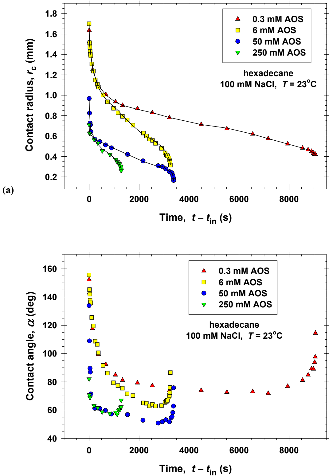
Figure 5. Effect of AOS concentration on the detachment of hexadecane drops from glass: Experimental data (a) for the contact radius, r_c , and (b) for the contact angle, \alpha , plotted vs. time; the initial moment, t_{\text{in}} , corresponds to the first experimental point. The NaCl concentration is 100 mM and the temperature is 23^\circ\text{C} .
