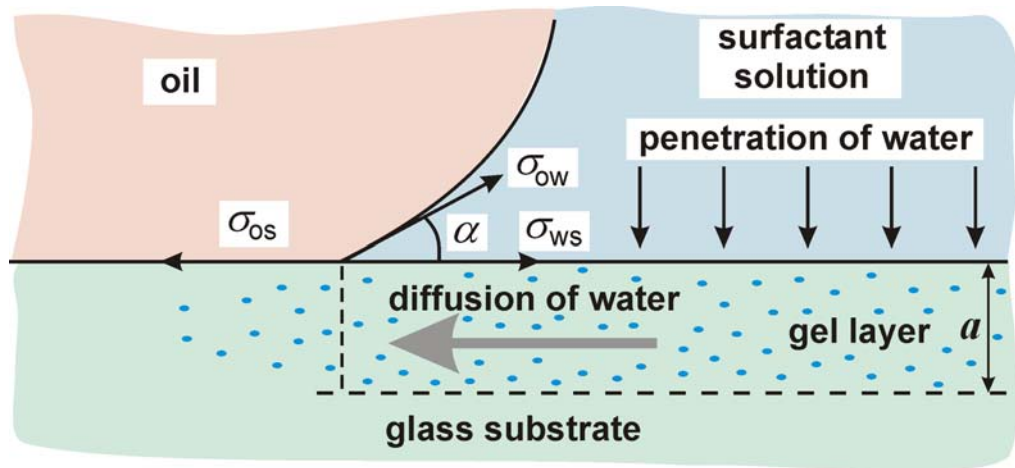
Figure 9. A possible model of the spontaneous detachment of an oil drop from a glass substrate in surfactant solution. Water molecules from the gel layer at the glass-water interface penetrate by diffusion the glass-oil interface (in the close vicinity of the contact line) and alter the local values of the two superficial tensions, \sigma_{ws} and \sigma_{os} , which, in their turn, affect the force balance at the contact line.
